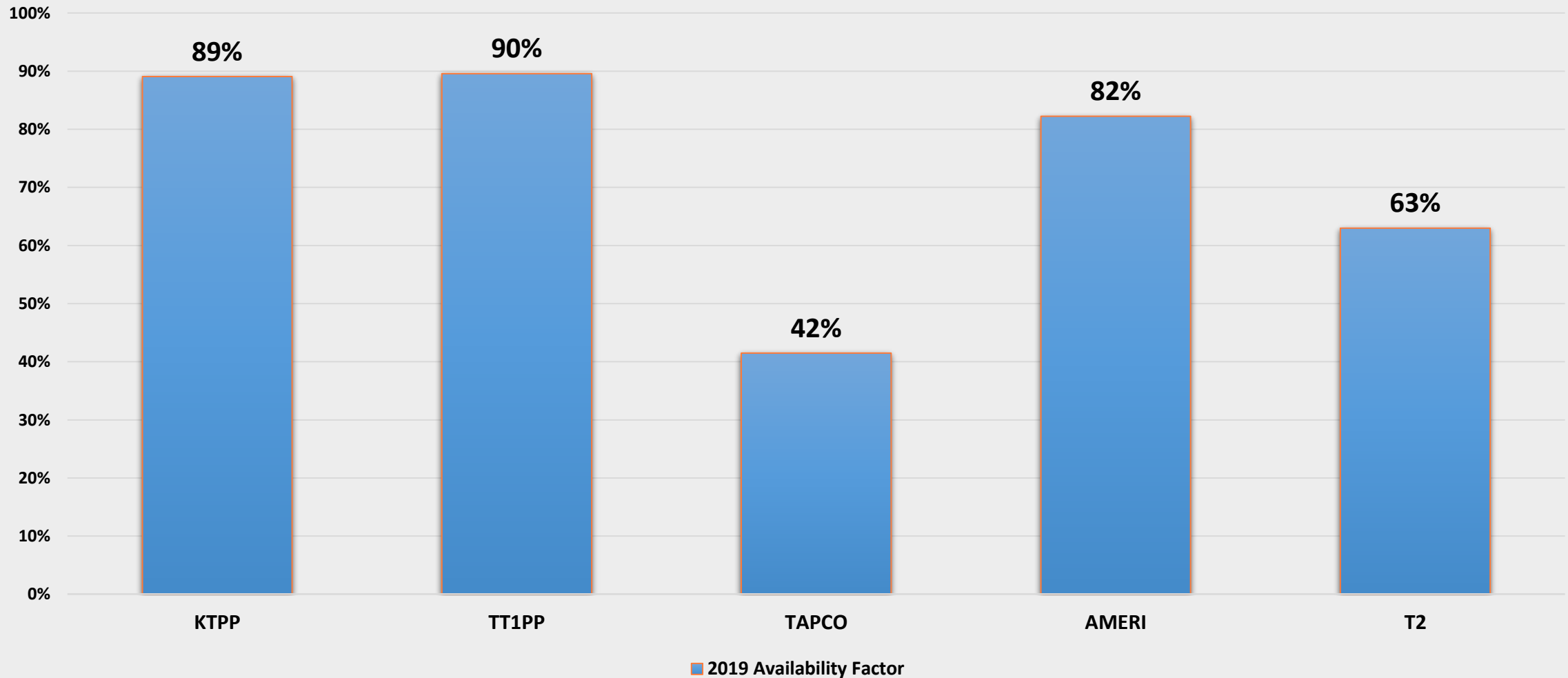
PLANT AVAILABILITY - DECEMBER 2019
